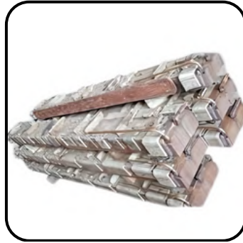
Lamination Yokes
