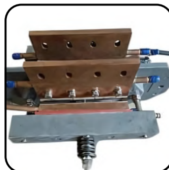
Furnace Change over Capacitor Cutoff Switches
